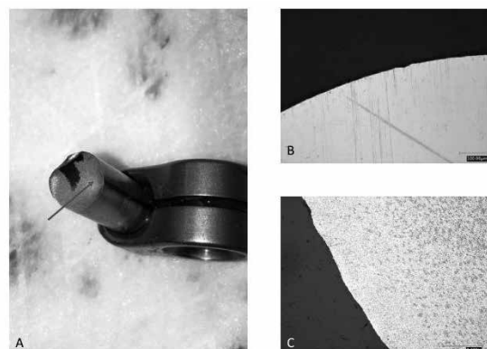
A) [left image] Fatigue fracture surface observed in operating room. Note red arrow indicating half-moon at the laser mark denoting fracture origin. B) [top right] Notch due to laser mark on CoCrMoC rod. C) [bottom right] Subsurface Ti alpha phase.
