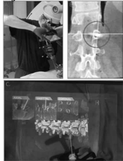
Figure 1. A. Surgeon wearing active 3D goggles for visualization of internal anatomy. B. Jamshidi needle position correlated to intraoperative scan. C. Virtual anatomy overlying cadaver as seen by surgeon through 3D goggles.
