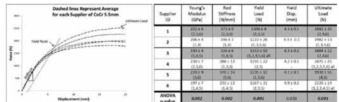
FIG: Load vs displacement curves. TABLE: Calculated values (mean ± standard deviation) with significantly different suppliers in parentheses below (ex: Supplier 1 Young's modulus was different than that of Suppliers 2, 3, 6). Significance set at p < 0.0083 .
